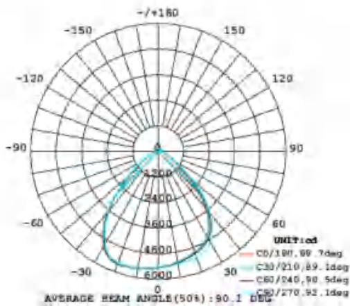
Beam angle 90°
