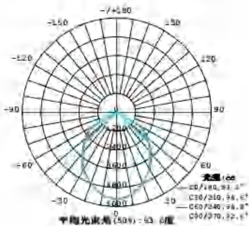
Beam angle 120°
